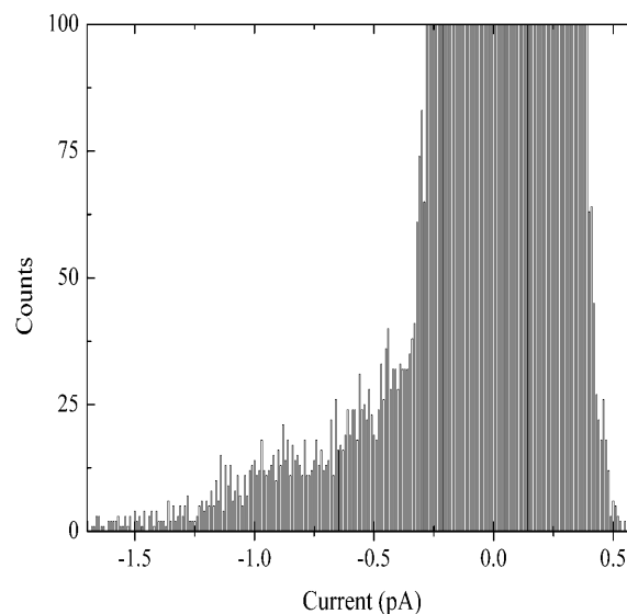
FIGURE 5 Accumulated all-points histogram of all records at 0 mV for the lecithin membrane with 30 mol % cholesterol at 25°C.
