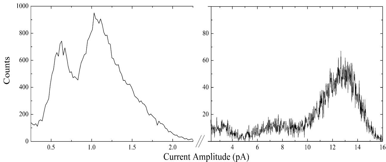
FIGURE 3 Accumulated all-points histogram of all records analyzed in the E. coli IOM bilayer at 25°C without cholesterol and AmB concentration of 100 \mu M. The solution used was 2 M KCl, 1mM CaCl 2 , and 10 mM Hepes at pH = 8.0. The applied membrane potential was 200 mV. The baseline at 0 current is not shown. In this case channel type V does not appear, but this histogram is shown because it corresponds to those conditions where channels are less likely to appear according to the assumption of sterols requirement.
